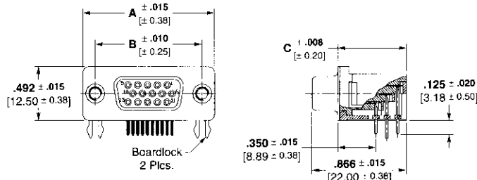
Right-Angle Receptacle
