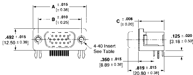
Right-Angle Plug
