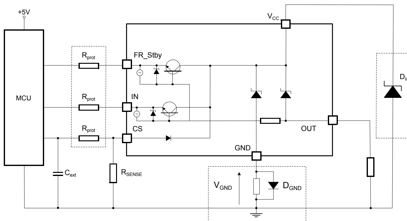
Figure 24. Application schematic
