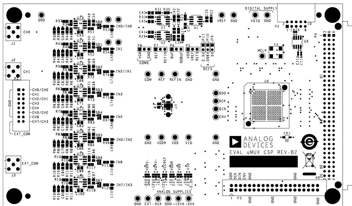
Figure 20. Top Side Silk-Screen
