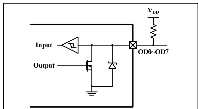
Figure 9 IS31O7325 Open-Drain I/O Ports Structure
