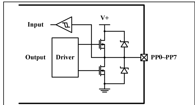
Figure 8 IS31O7325 Push-Pull I/O Ports Structure
