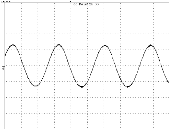
Figure 9: Input Terminal Ripple Current, i_o , at full rated output current and nominal input voltage with 12\mu\text{H} source impedance and 33\mu\text{F} electrolytic capacitor (100mA/div, 1us/div)
