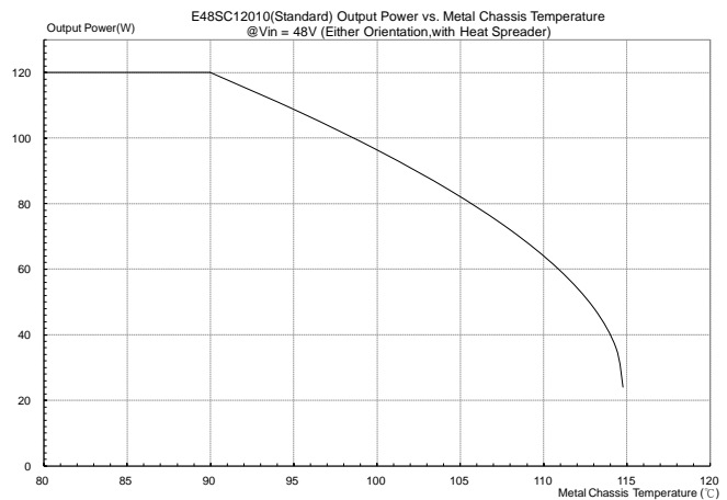
Figure 24: Output power vs. Metal chassis temperature @Vin=48V (Either orientation, with heat spreader)
