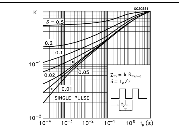
Figure 3. Thermal impedance for TO-220FP and I 2 PAKFP
