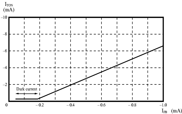
Fig.4 Feedback Current versus Charging Current Characteristics
