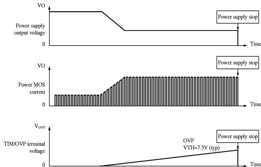
Fig. 10 Timer Latch Basic Operation
