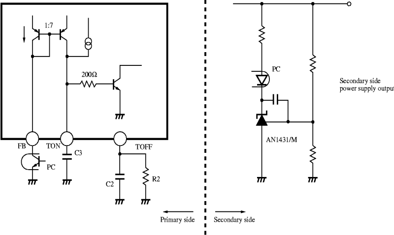
Fig.3 Power Supply Output Control System
