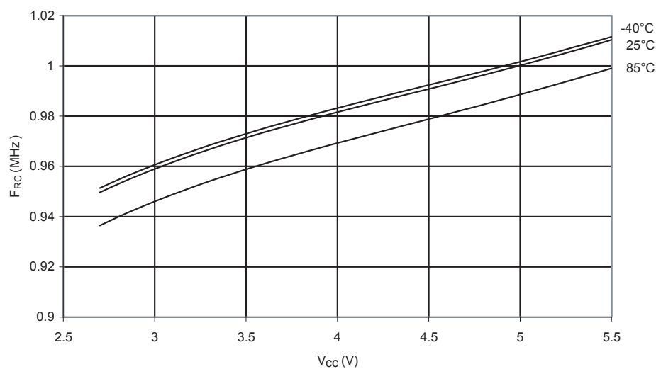
Figure 203. Calibrated 1 MHz RC Oscillator Frequency vs. V_{CC}
