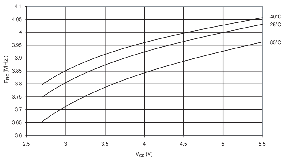
Figure 209. Calibrated 4 MHz RC Oscillator Frequency vs. V_{CC}
