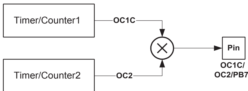
Figure 72. Output Compare Modulator, Block Diagram
