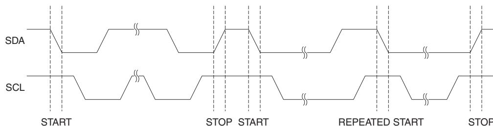
Figure 88. START, REPEATED START, and STOP Conditions
