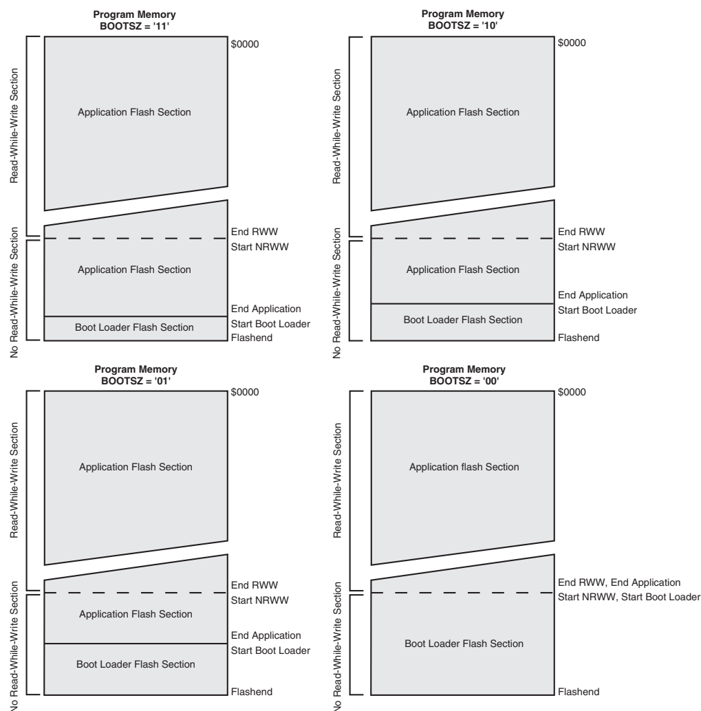
Figure 136. Memory Sections (1)
