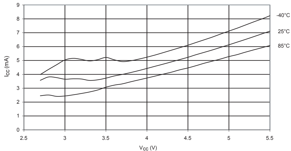
Figure 218. Programming Current vs. V_{CC}
