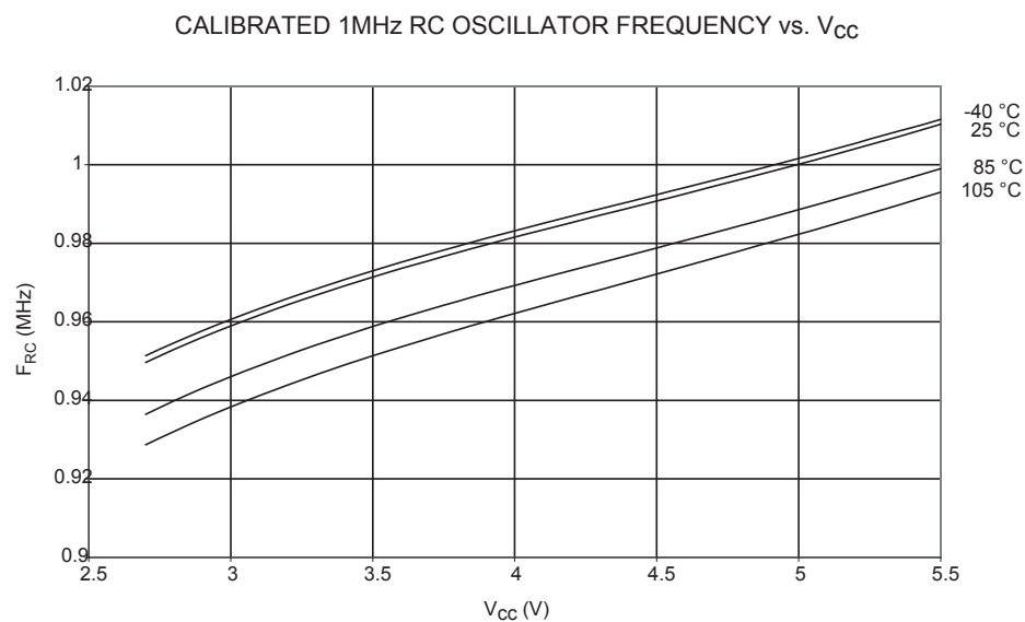
Figure 249. 1 MHz RC Oscillator Frequency vs. V_{CC}
