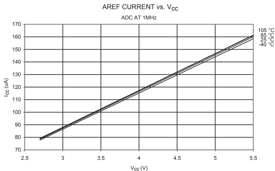
Figure 255. 1 MHz Aref Current vs. V_{CC}
