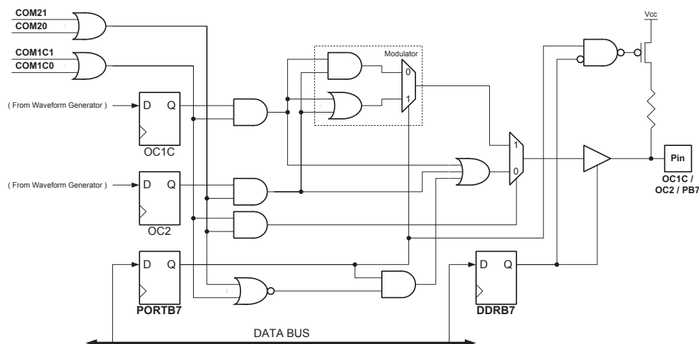
Figure 73. Output Compare Modulator, Schematic
