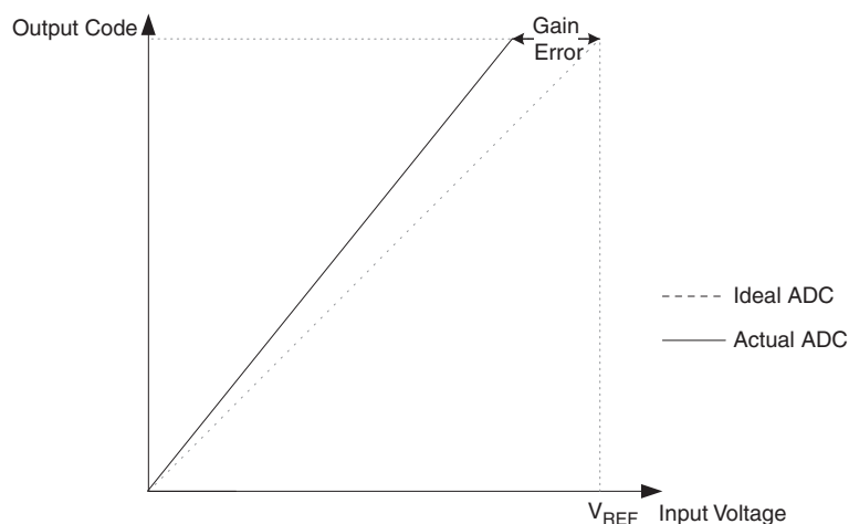
Figure 118. Gain Error
