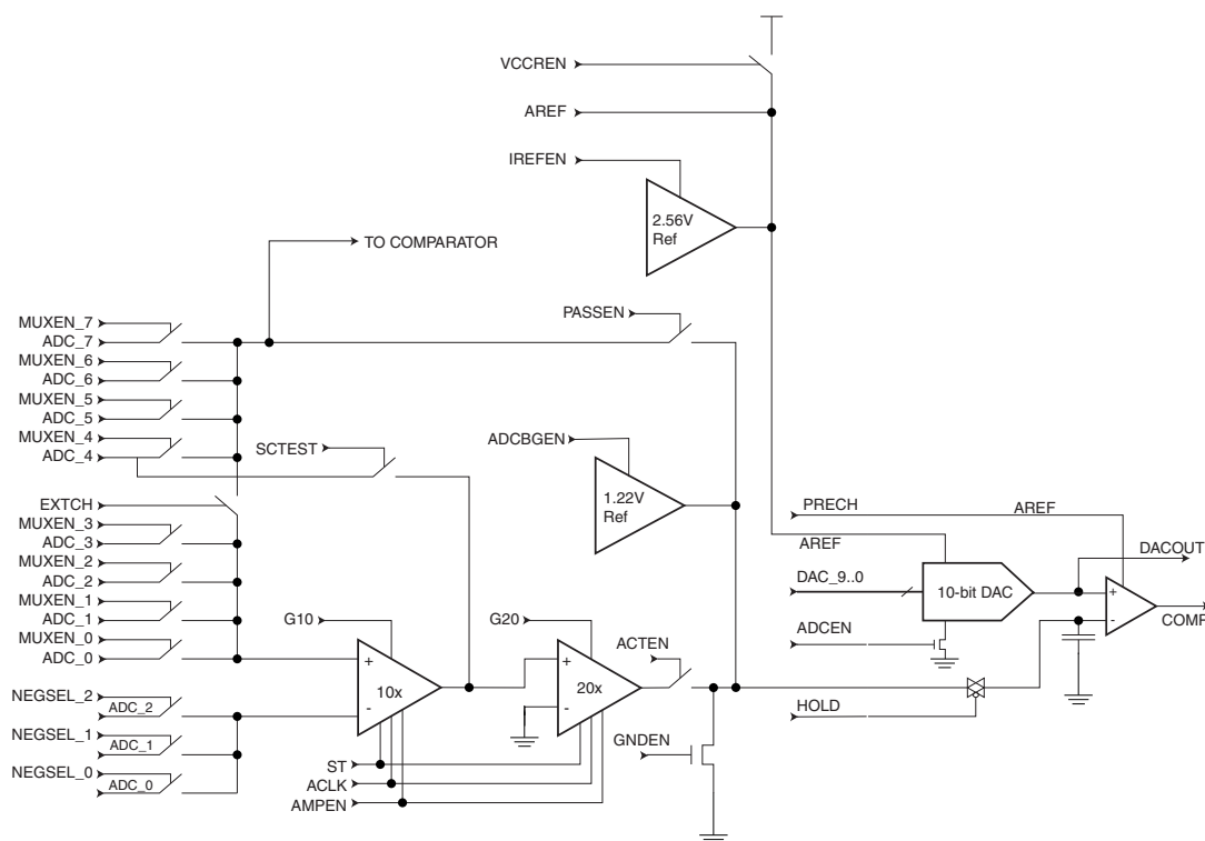
Figure 134. Analog to Digital Converter
