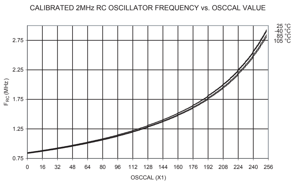
Figure 252. 2 MHz RC Oscillator Frequency vs. OSCCAL
