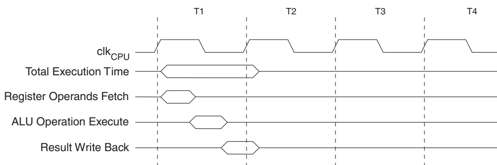
Figure 7. Single Cycle ALU Operation
