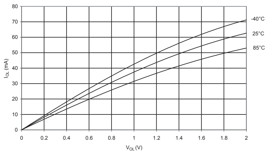
Figure 190. I/O Pin Sink Current vs. Output Voltage ( V_{CC} = 5V )
