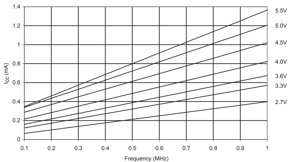
Figure 170. Idle Supply Current vs. Frequency (0.1 MHz - 1.0 MHz)
