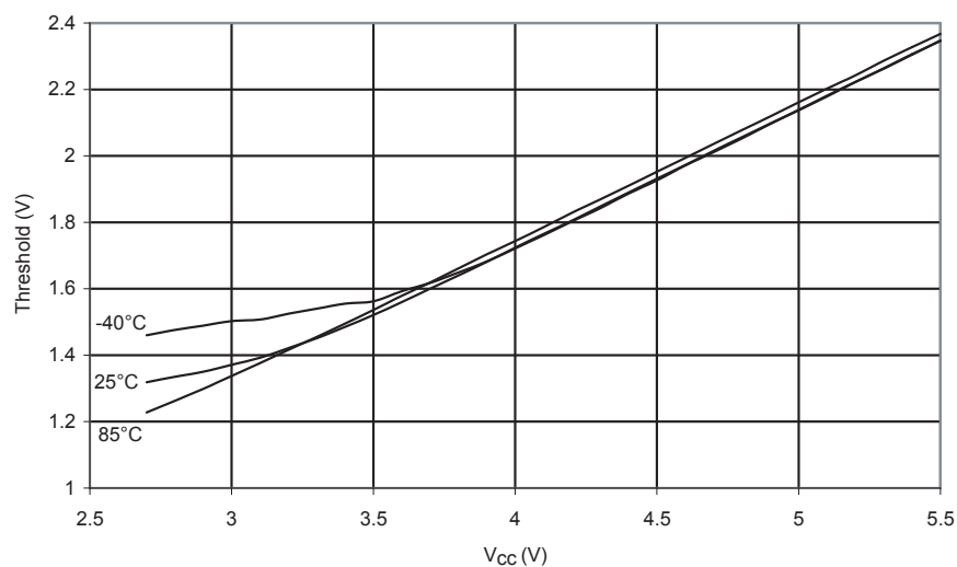
Figure 195. Reset Input Threshold Voltage vs. V_{CC} ( V_{IH} , Reset Pin Read as '1')
