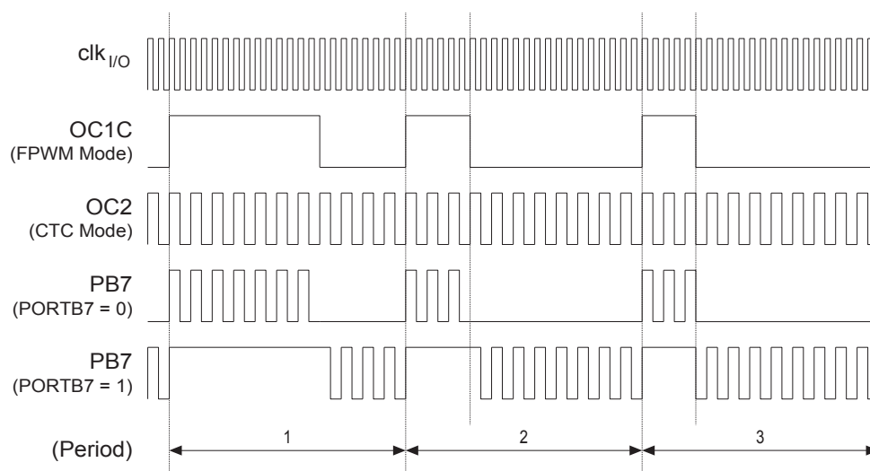
Figure 74. Output Compare Modulator, Timing Diagram
