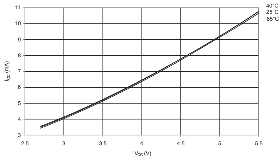
Figure 175. Idle Supply Current vs. V_{CC} (Internal RC Oscillator, 8 MHz)
