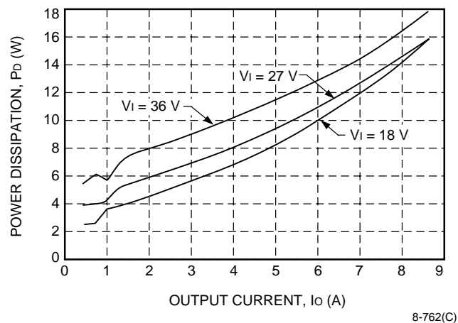
Figure 22. Power Dissipation as Heat vs. Output Current
