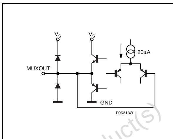
Figure 23. PINS: 6, 8
