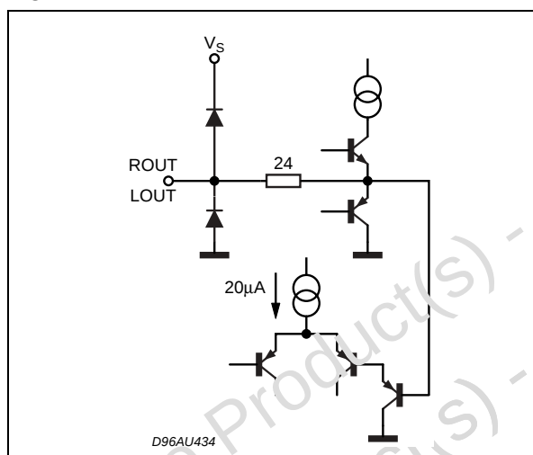
Figure 21. PINS: 26, 27
