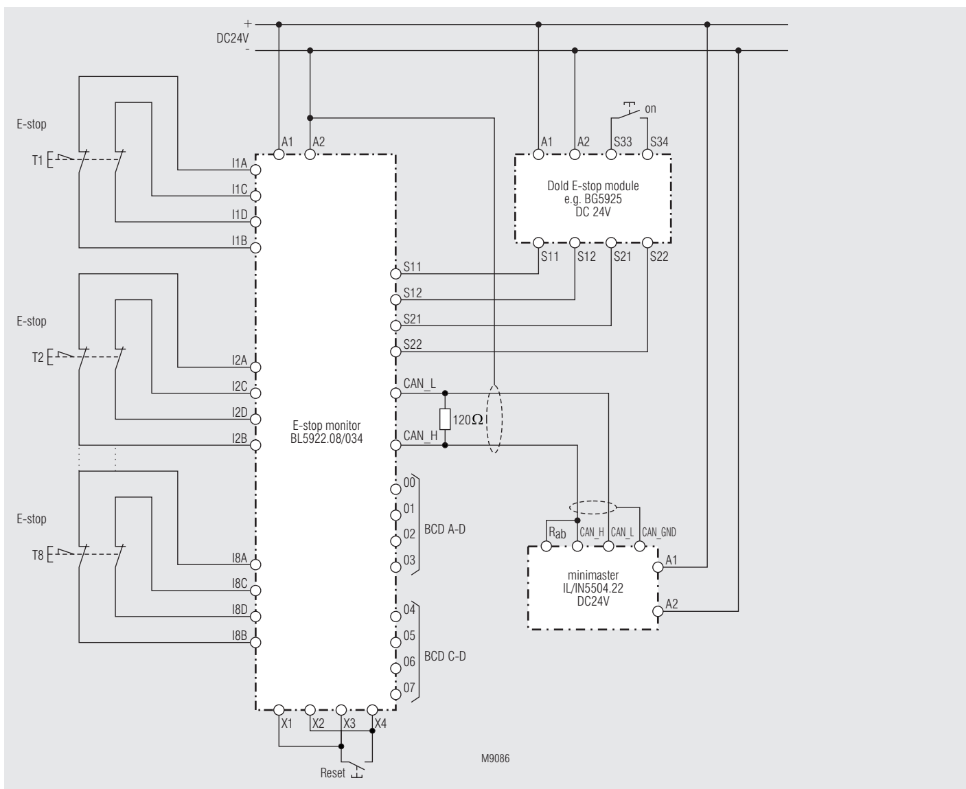
Pic 8: Monitoring of 8 e-stop buttons with e-stop monitor, 2-channel connection, 2-channel monitoring cross fault monitoring with CANopen minimaster IL 5504, IN 5504
