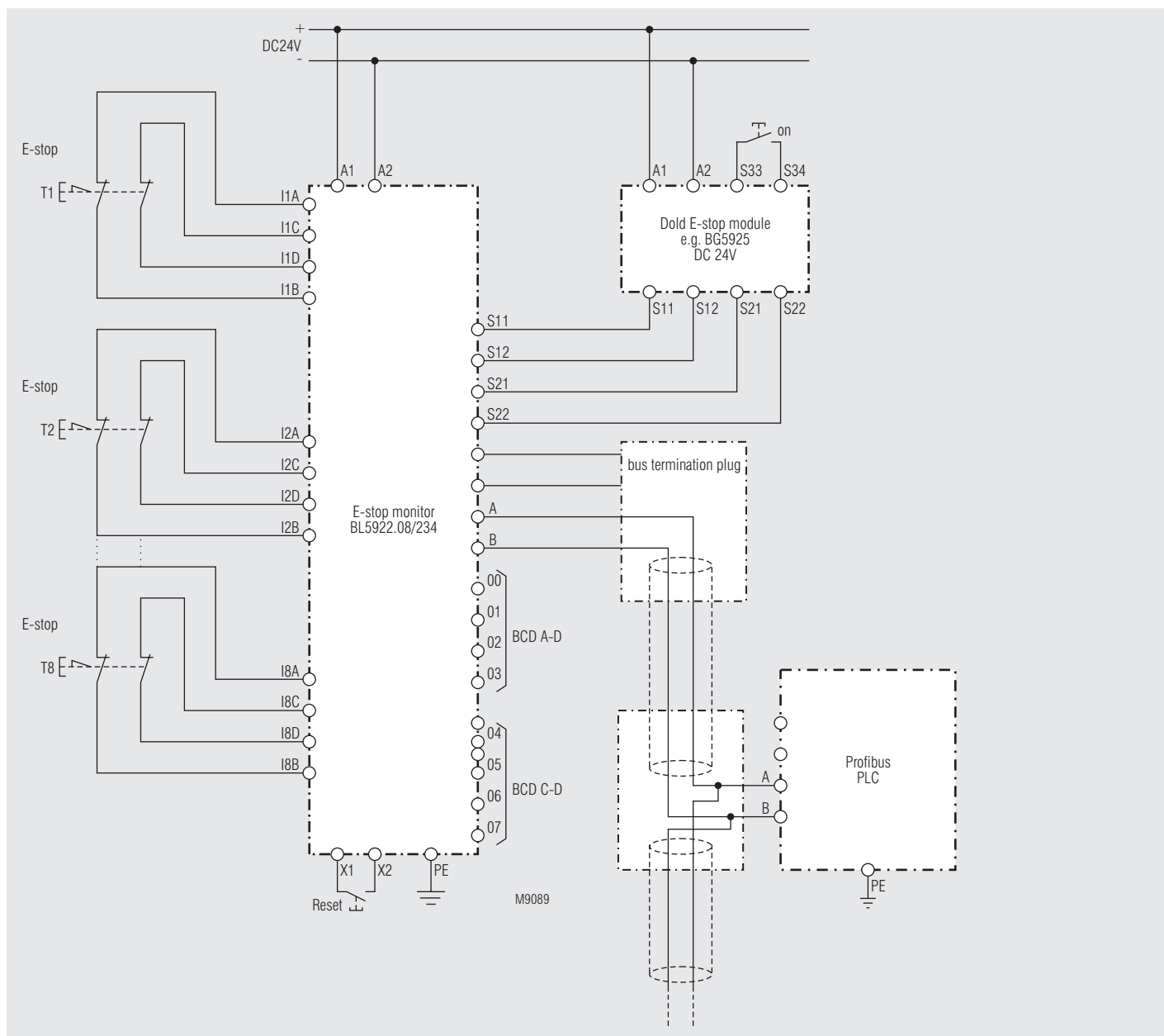
Pic 9: Monitoring of 8 e-stop buttons with e-stop monitor, 2-channel connection, 2-channel monitoring cross fault monitoring with Profibus DP-PLC
