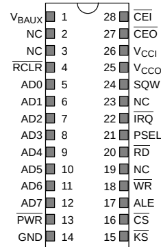
DS1693 28-PIN ENCAPSULATED PACKAGE (740 MIL)
