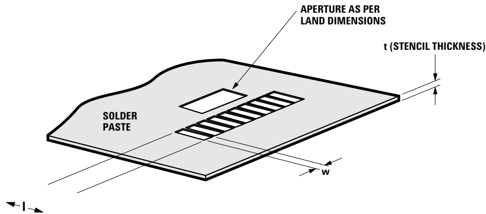
Figure 4.0. Solder paste stencil aperture.
