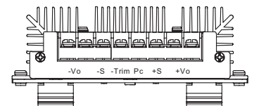
Back View
