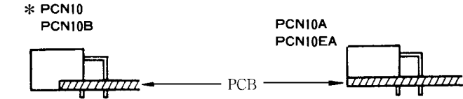
* The receptacle double-row right angle type indicates the type of PCN10A type.
