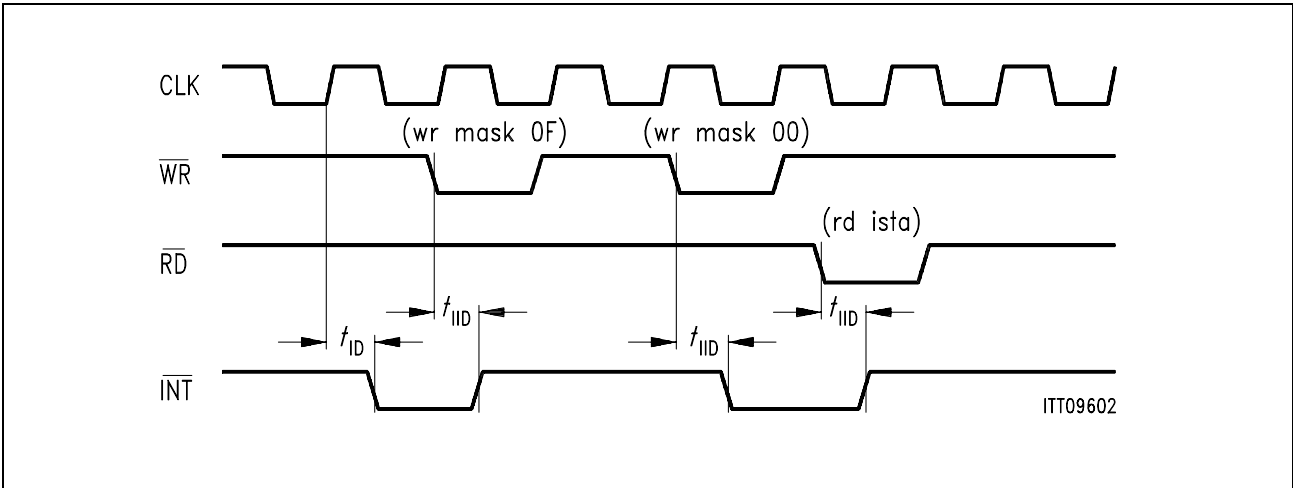
Figure 18 Interrupt Timing
