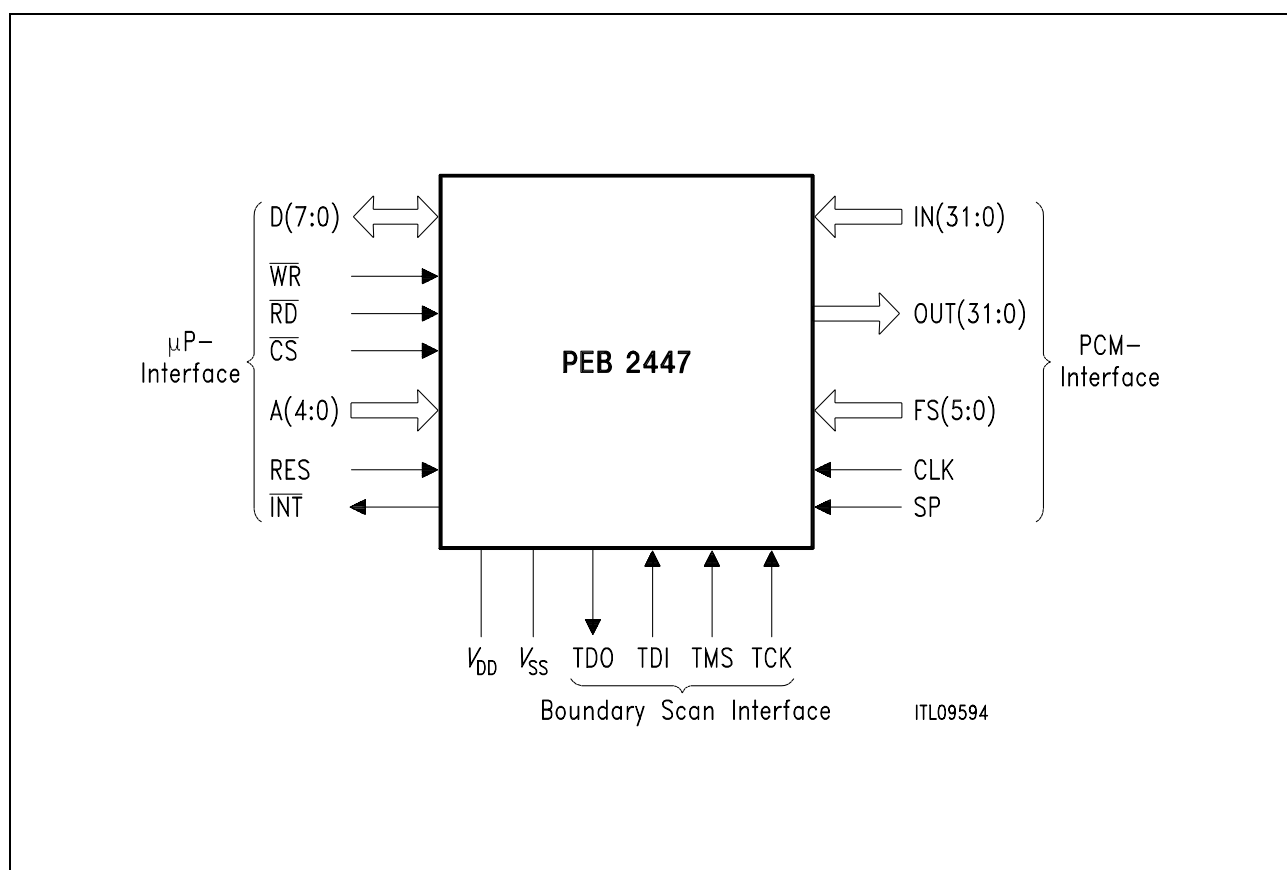
Figure 1 Functional Symbol
