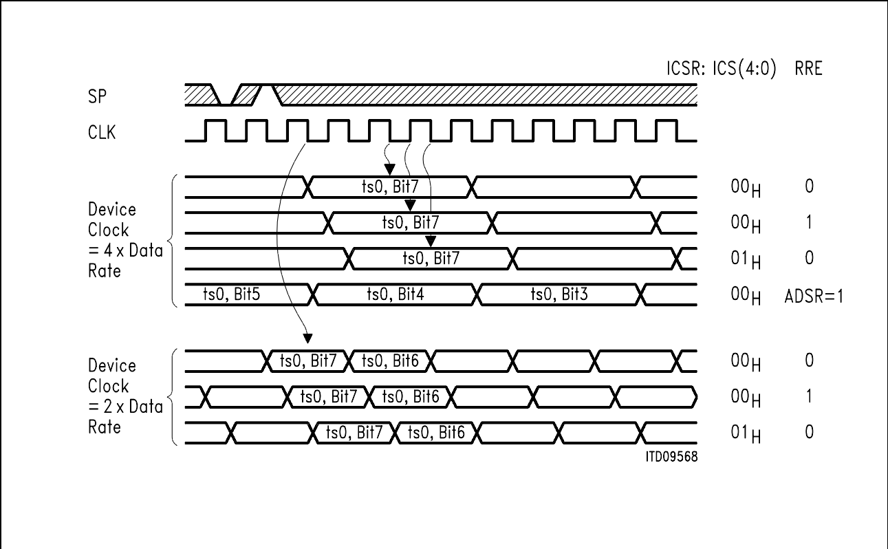
Figure 9 Input Timing
