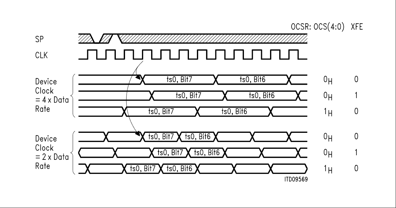
Figure 10 Output Timing
