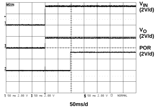
FIGURE 10. START-UP 2
