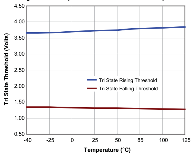
Fig 11. PWM Input Tristate Threshold vs. Temperature
