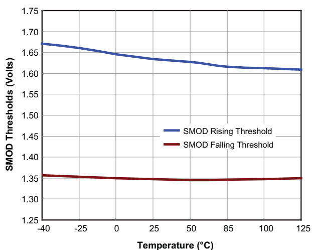
Fig 14. SMOD Input Threshold vs. Temperature
