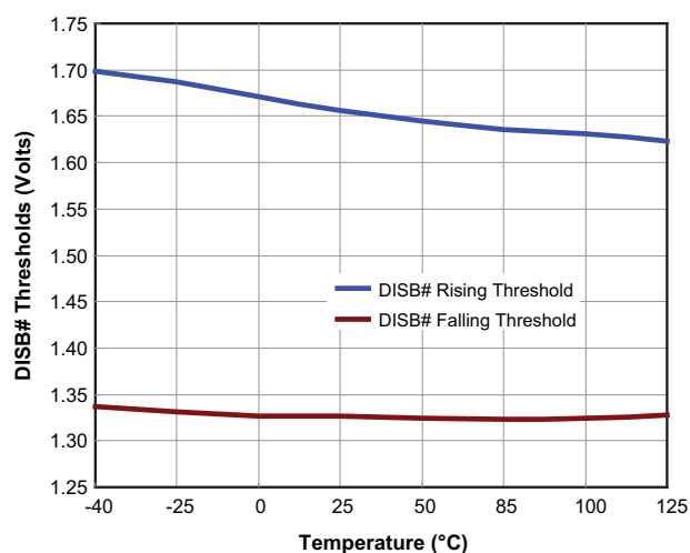
Fig 13. DISB# Input Threshold vs. Temperature
