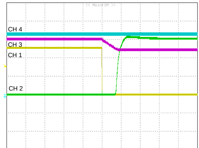
Figure 4: Oring for one feed loss (500µS/div): CH1: IinA (2A/div) CH2: IinB (2A/div). CH3: VRTN_OUT reference to -48V_OUT (10V/div). CH4: VMGMT_PWR (1V/div).
