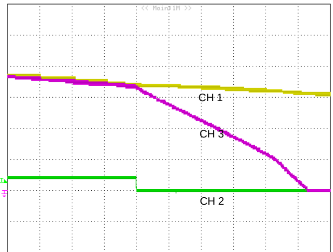
Figure 2: Input voltage turn-off threshold (2mS/div): CH1: Vin (VRTN_AF reference to -48V_AF, 10V/div). CH2: Iin (-48V_AF, 2A/div). CH3: VRTN_OUT reference to -48V_OUT (10V/div).
