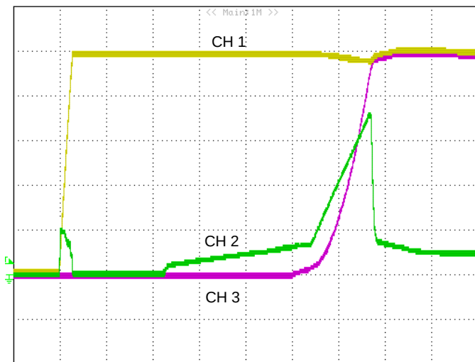
Figure 3: Inrush current (2mS/div): CH1: Vin (VRTN_AF reference to -48V_AF, 10V/div). CH2: Iin (-48V_AF, 2A/div). CH3: VRTN_OUT reference to -48V_OUT (10V/div).
