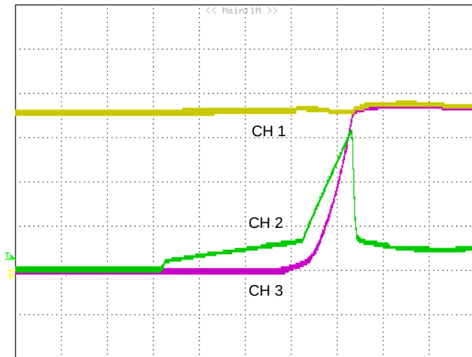
Figure 1: Input voltage turn-on threshold (2mS/div): CH1: Vin (VRTN_AF reference to -48V_AF, 10V/div). CH2: Iin (-48V_AF, 2A/div). CH3: VRTN_OUT reference to -48V_OUT (10V/div).
