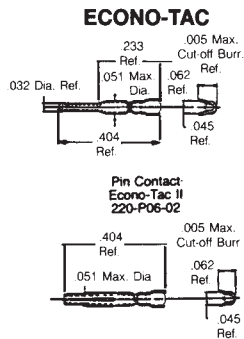
Pin Contact Econo-Tac II 220-P02-02
