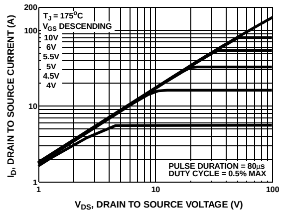
Figure 2. Output Characteristics
