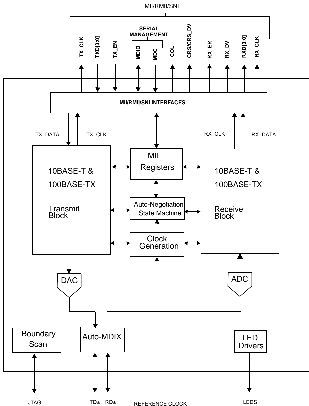
Figure 1. DP83848YB Functional Block Diagram
