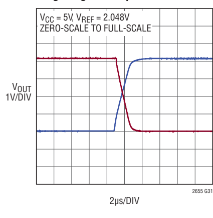
Large-Signal Response
