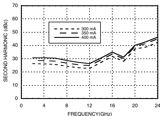
Second Harmonics vs. I_{dd} @ P_{out} = 18 \text{ dBm} , V_{gg} = 3.5\text{V}
