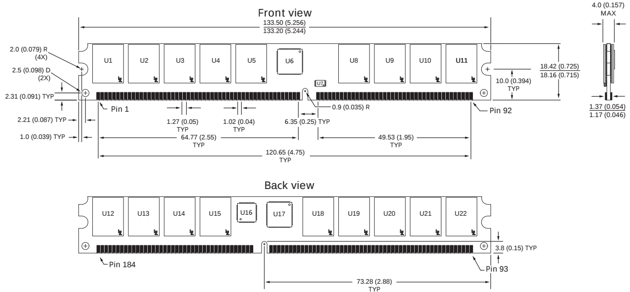
Figure 3: 184-Pin DDR VLP RDIMM
