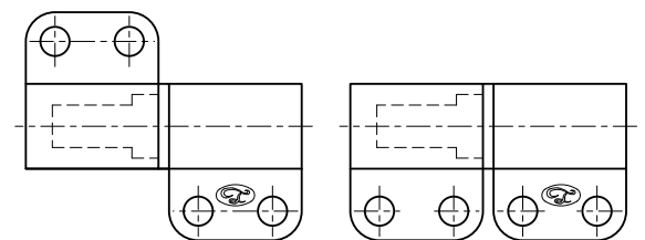
逆組 (納入形態) Reverse setting (at delivery)
