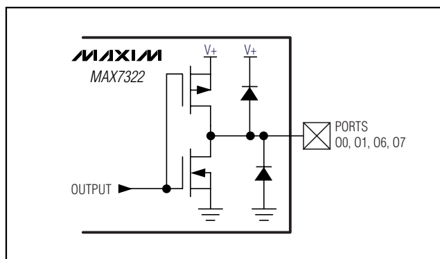
Figure 9. MAX7322 Push-Pull Output Port Structure
