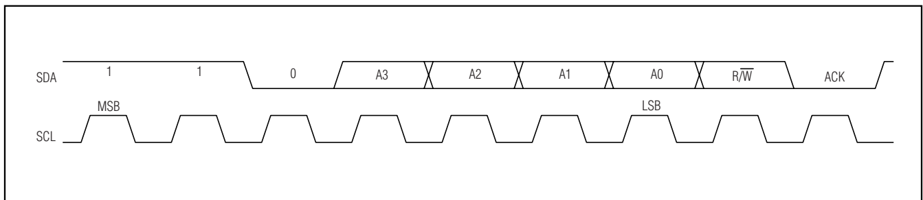
Figure 5. Slave Address
