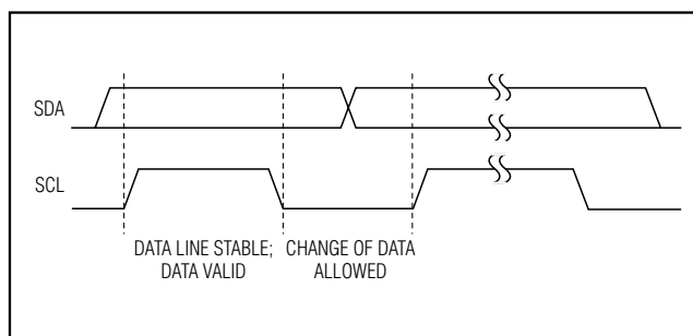
Figure 3. Bit Transfer
