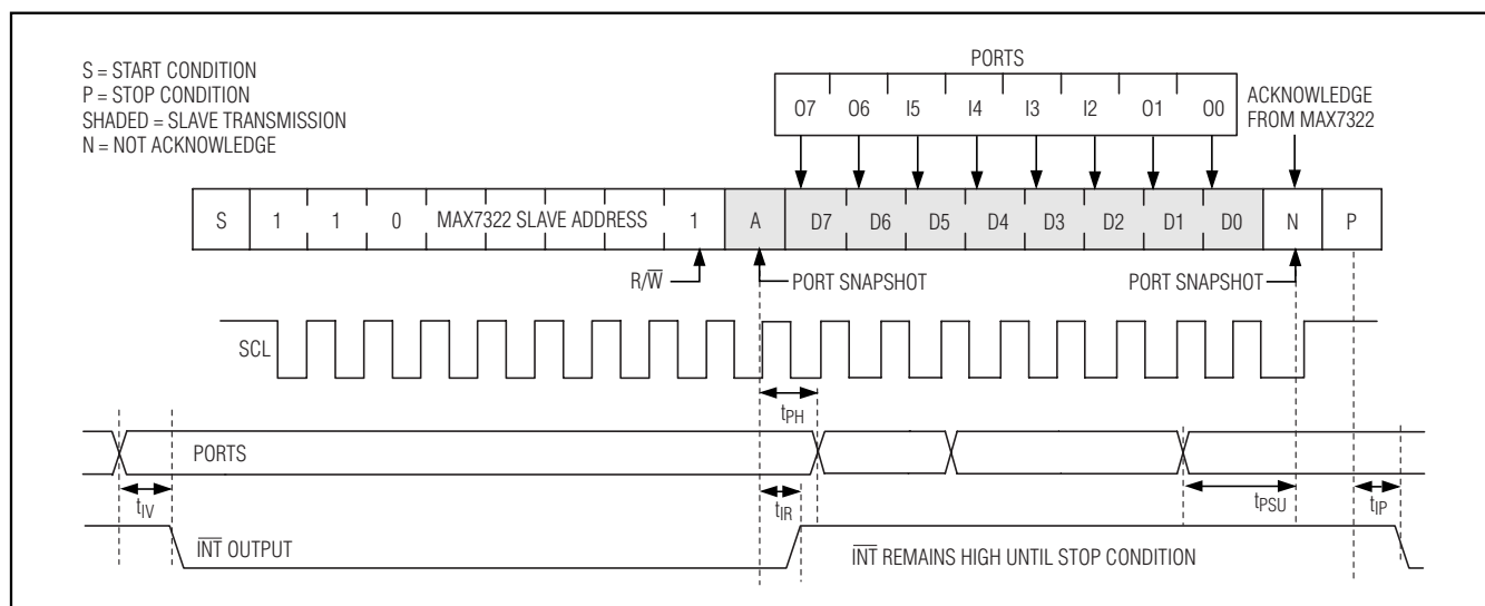
Figure 6. Reading from the MAX7322 (1 Data Byte)
