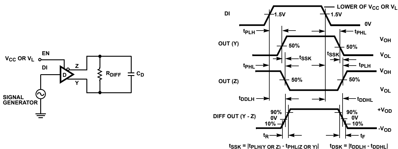
FIGURE 5A. TEST CIRCUIT
