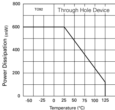
Power Derating
