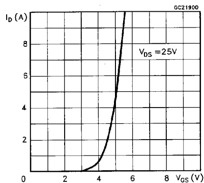
Transfer Characteristics
