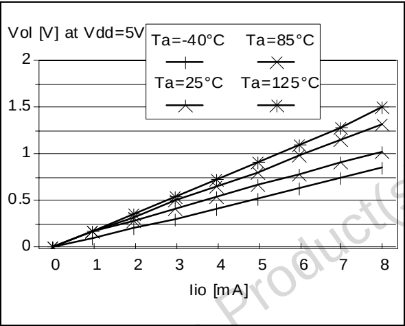
Figure 88. Typical V_{OL} at V_{DD}=5V ( \overline{RESET} )
