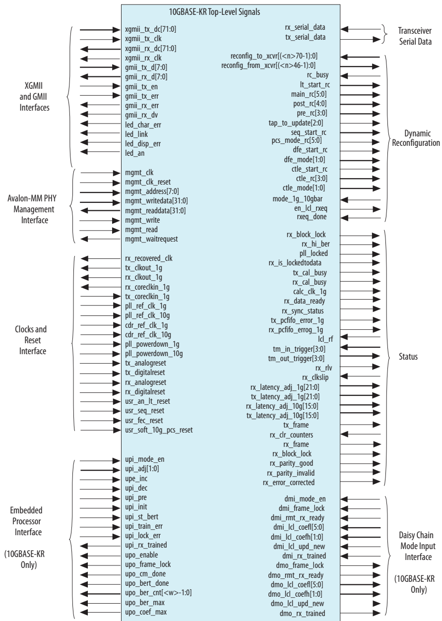
Figure 4-11: 10GBASE-KR Top-Level Signals
