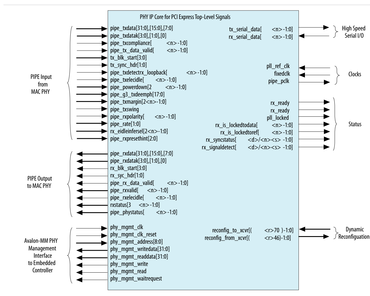
Figure 8-3: Top-Level Signals of the PHY IP Core for PCI Express
