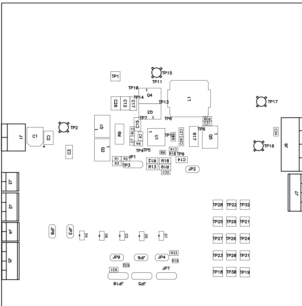
Figure 9. Top Assembly
