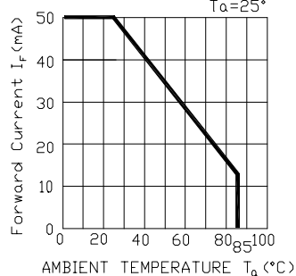
Forward Current Derating Curve T_a=25^\circ
