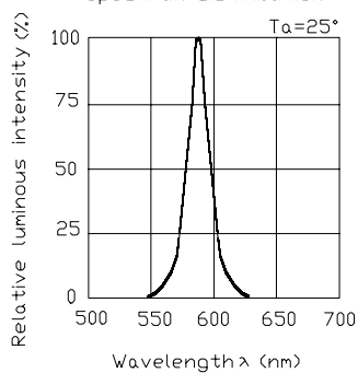
Spectrum Distribution T_a=25^\circ
