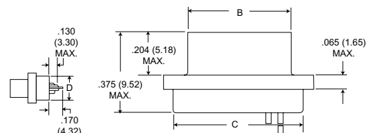
Solder Pot
