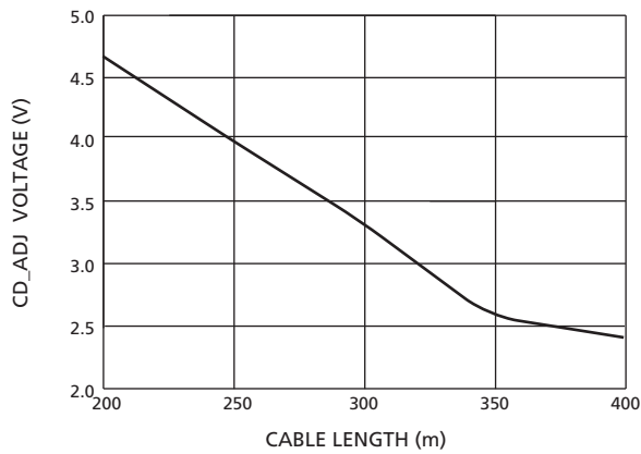
Figure 2-4: Carrier Detect Adjust Voltage Threshold Characteristics
