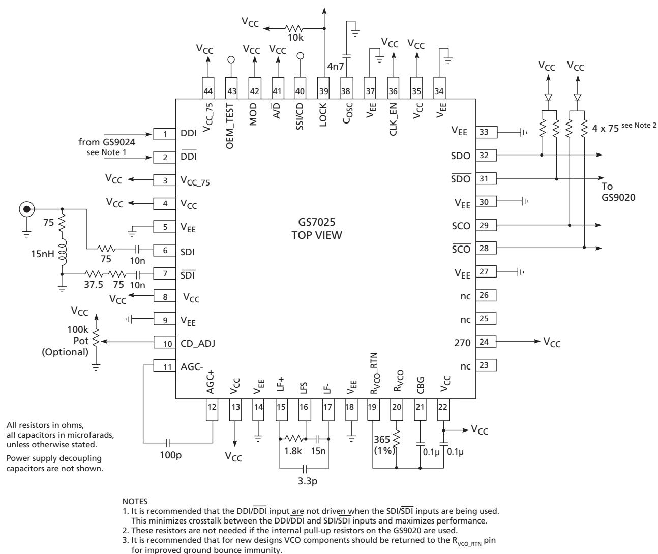
Figure 4-1: GS7025 Typical Application Circuit
