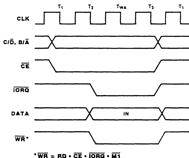
Figure 12. Write Cycle Timing
