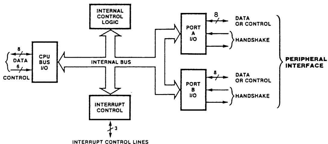
Figure 4. Block Diagram
