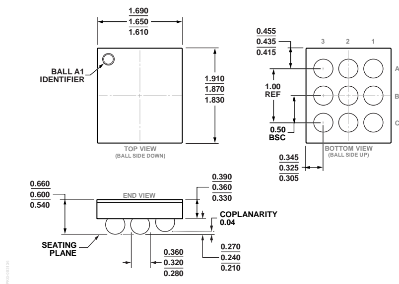
Figure 44. 9-Ball Wafer Level Chip Scale Package [WLCSP] 1.65 mm x 1.87 mm Body (CB-9-6) Dimensions shown in millimeters
