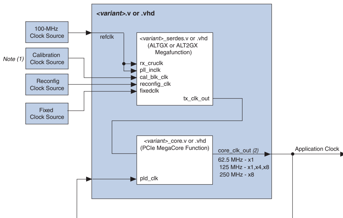
Figure 7-4. Arria II GX, Arria II GZ, Cyclone IV GX, HardCopy IV GX, Stratix IV GX x1, x4, or x8 100 MHz Reference Clock
