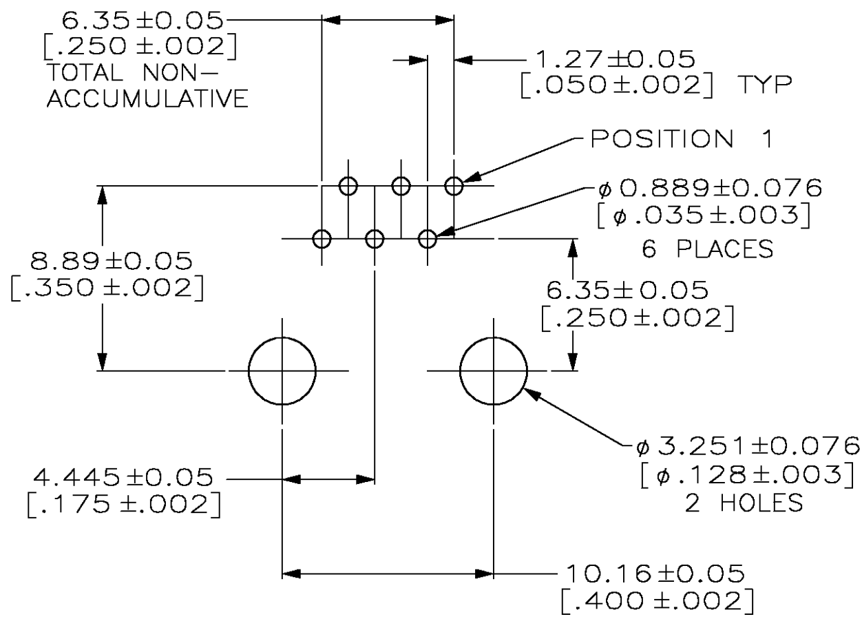
SUGGESTED PC BOARD LAYOUT CIRCUIT SIDE SHOWN
