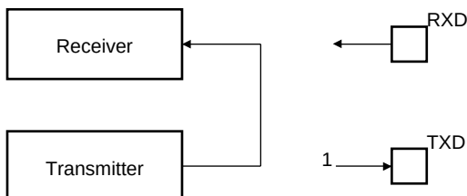
Figure 33-30. Local Loopback Mode Configuration
