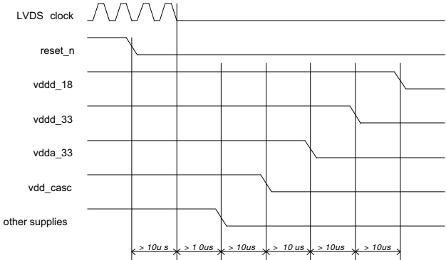
Figure 18. Power-down Sequence
