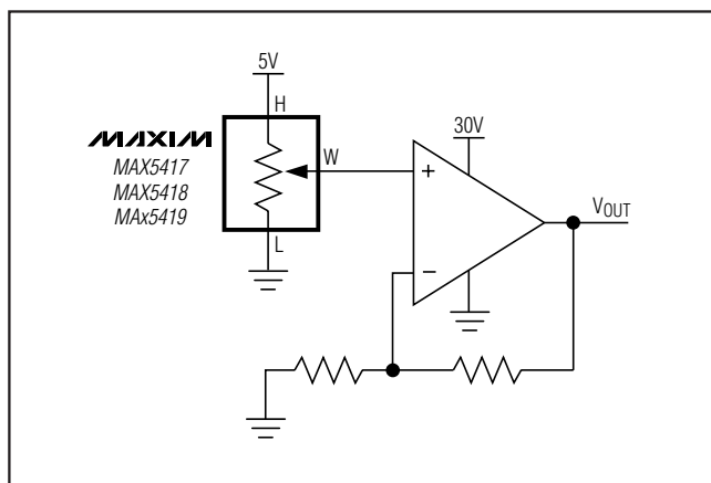
Figure 9. Positive LCD Bias Control Using a Voltage-Diver
