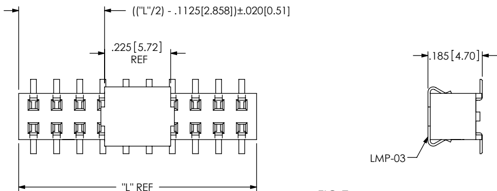
-M: METAL PICK & PLACE PAD ONLY AVAILABLE ON -DV (MMS-140-02-XXX-DV-M SHOWN) (DIFFERENT AS SHOWN, OTHERWISE SAME AS FIG 1)
