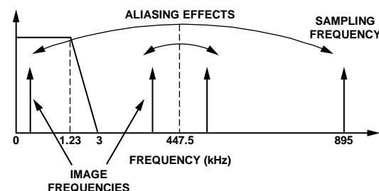
Figure 38. Aliasing Effect
