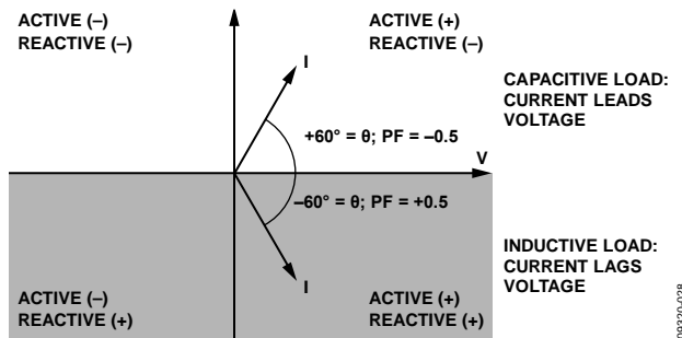
Figure 59. Capacitive and Inductive Loads
