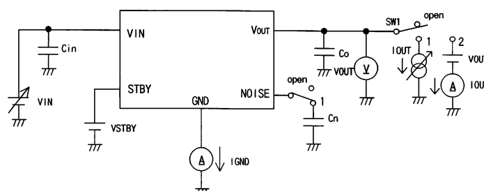
Fig.2 TEST CIRCUIT
