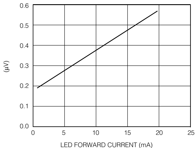
Figure 16. LED Offset Voltage vs. LED Current
