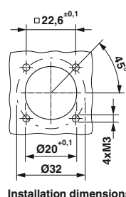
Installation dimensions
