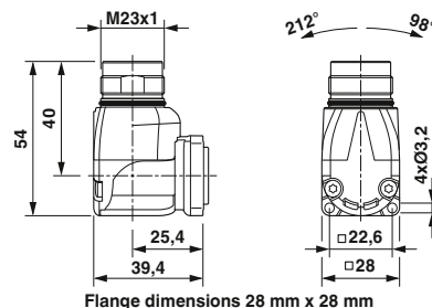
Flange dimensions 28 mm x 28 mm
