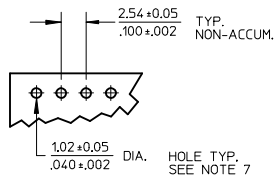
TYP. HOLE PATTERN FOR 1.57/.062 THK. PCB
