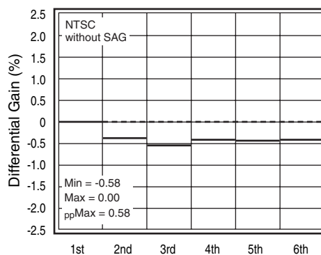
Figure 6. Differential Gain
