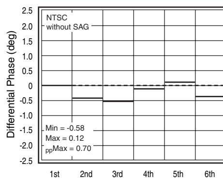
Figure 8. Differential Phase
